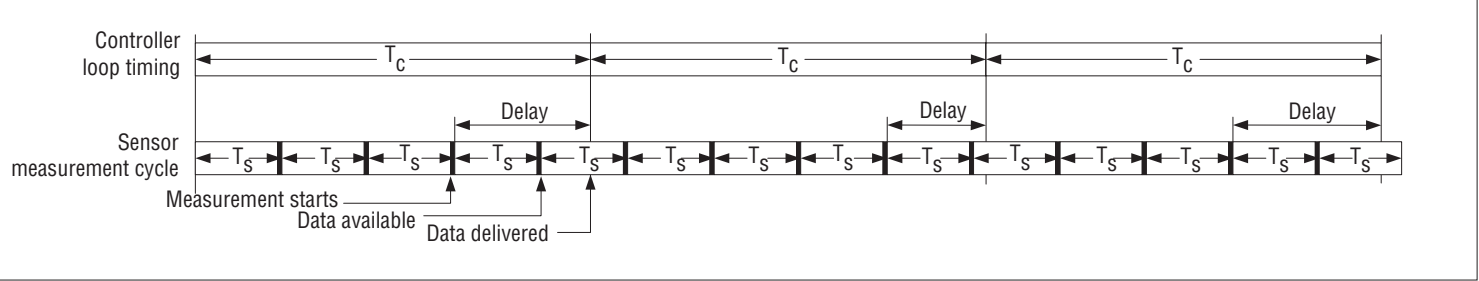
Fig. 12: Asynchronous SSI Interface
