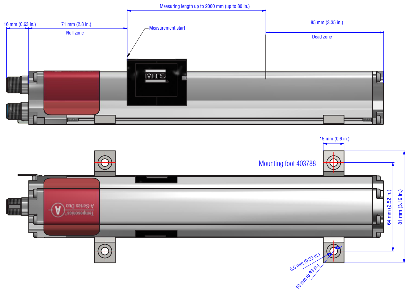
Fig. 3: Dual Channel linear encoder dimension reference
