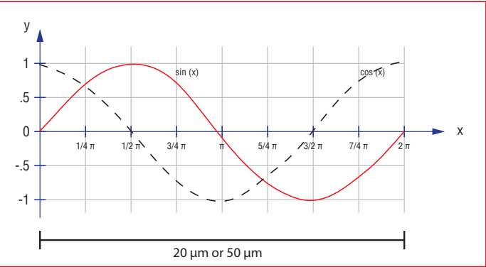
Fig. 8: Signal period
