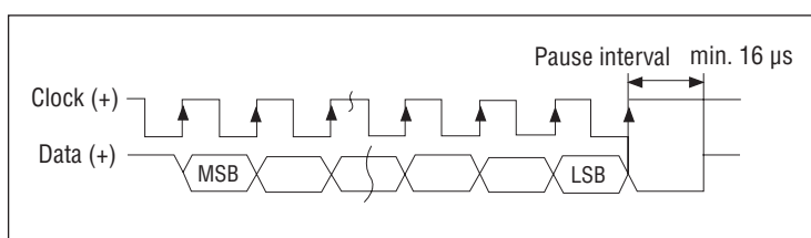
Fig. 9: Timing diagram
