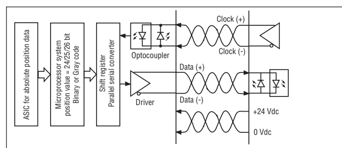
Fig. 11: Logic diagram
