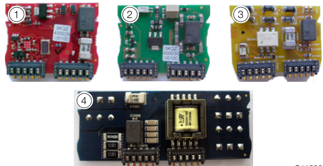
Fig. 30: Plug-in cards
