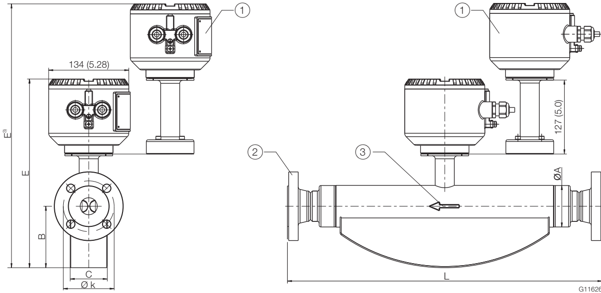
Fig. 22 ① Option "extended tower length or option "pressure rating of the pressure sensor housing" ② Flange in accordance with EN 1092-1, ASME B16.5, ISO 7005 (connection dimensions for ASME flanges acc. to ASME B16.5 (ANSI)) ③ Flow direction
