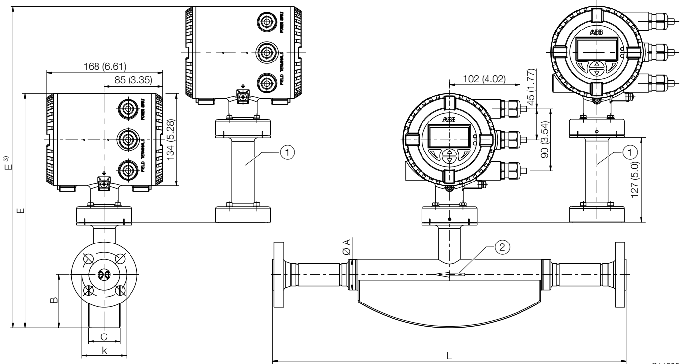
Fig. 20: Devices in integral mount design, tolerance for dimension L: +0 / -3 mm (+0 / -0.018 inch)
