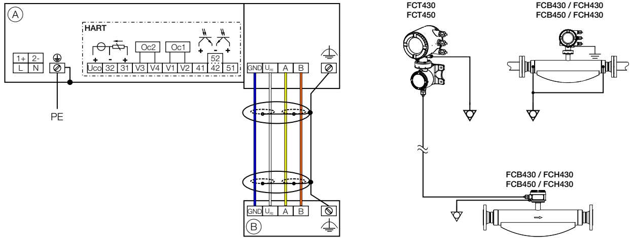
Fig. 31: (A) Transmitter (B) Sensor
