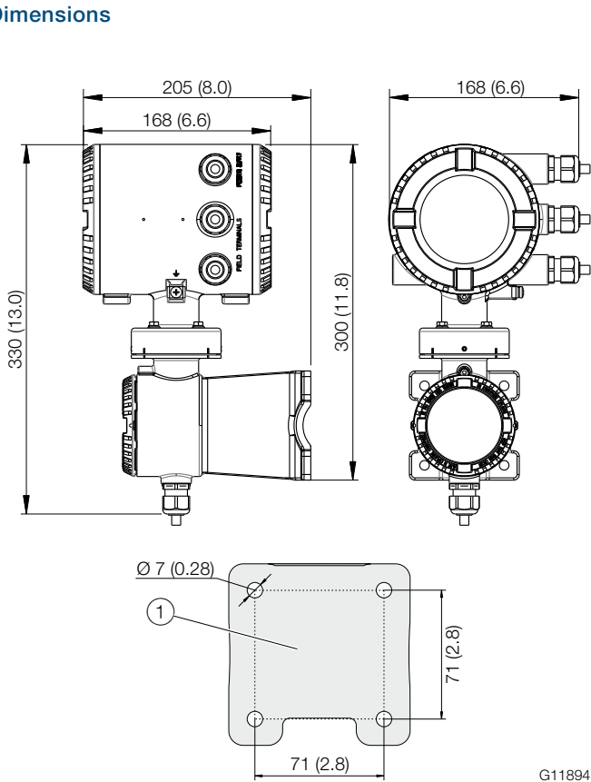
Fig. 44: Mounting dimensions of double-compartment housing
