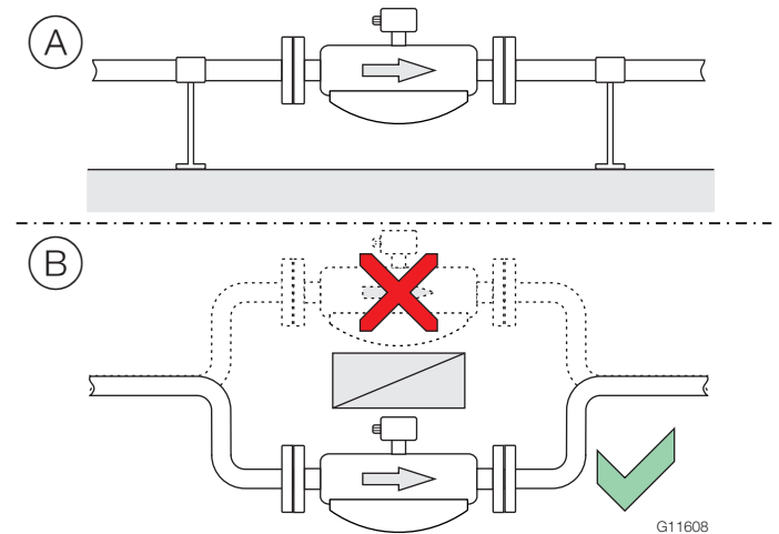
Fig. 5 Horizontal installation
