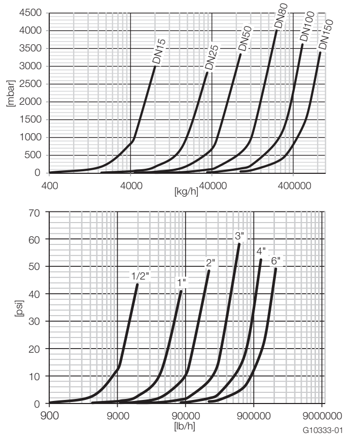
Fig. 11: Pressure loss curve (measured with water, viscosity: 1 mPas)
