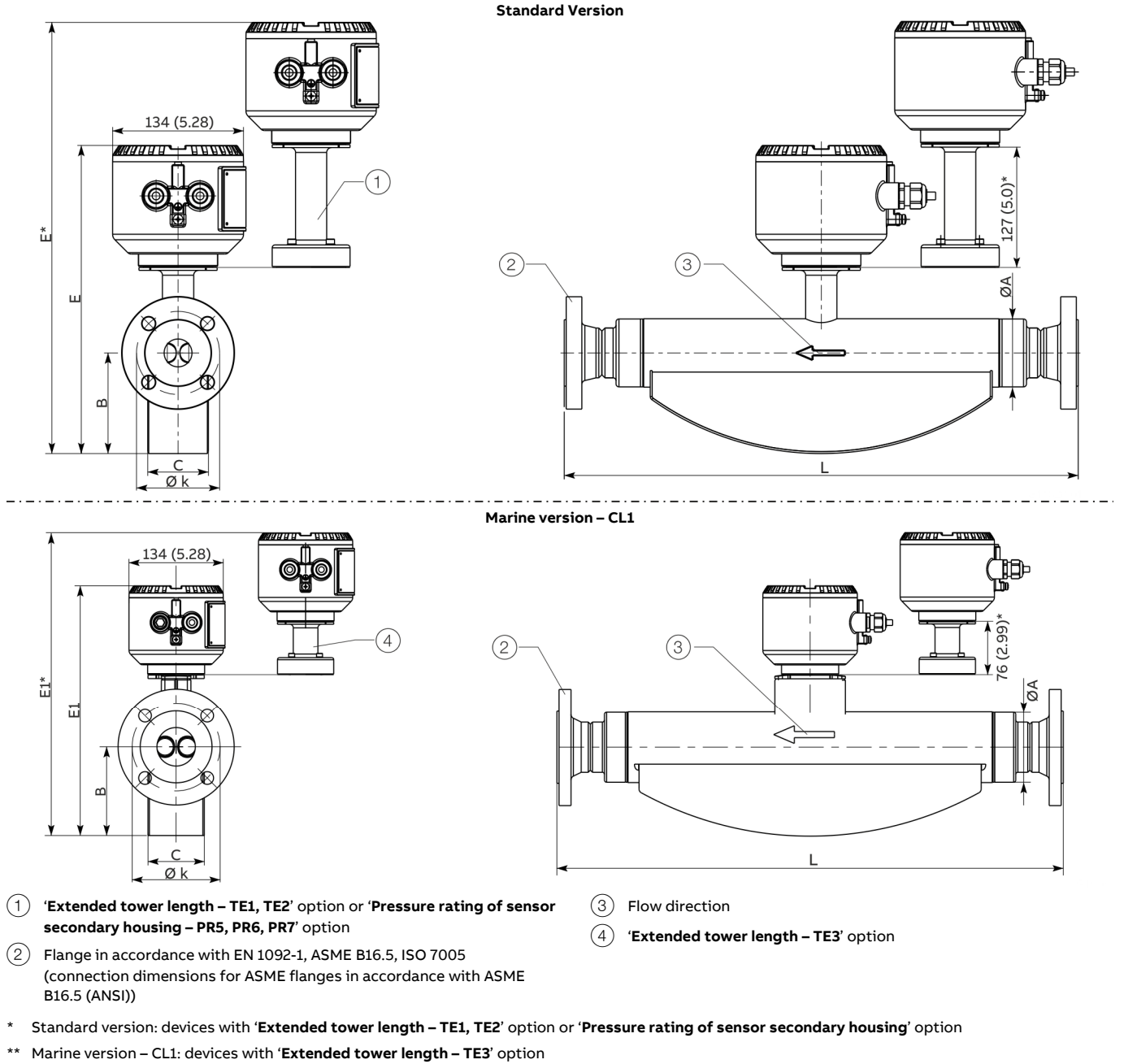
Figure 6: Remote mount design
